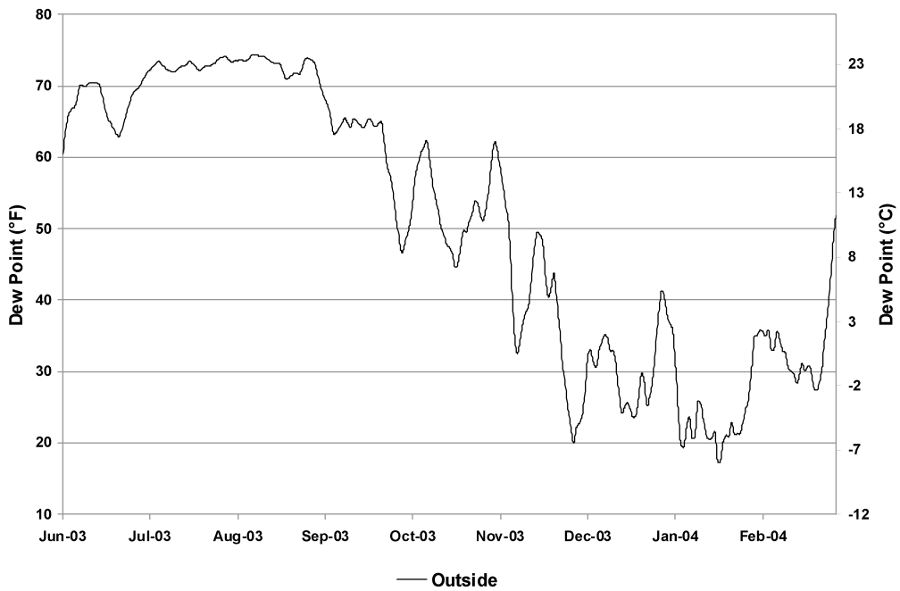
Figure 6 Outside air dew-point temperatures for Phase II.
